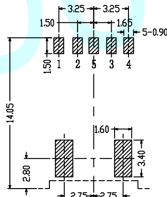
Recommend PCB Layout (Top View) Tolerance : ±0.05
