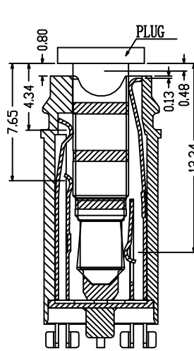
SBC :A-A Image Of Plug Match With Contact Point
