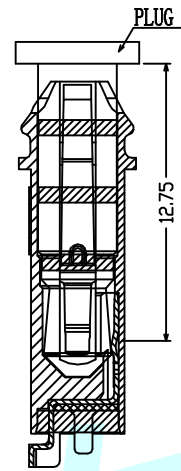
SBC :B-B Image Of Plug Match With Contact Point
