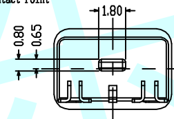
SBC :B-B Image Of Plug Match With Contact Point
