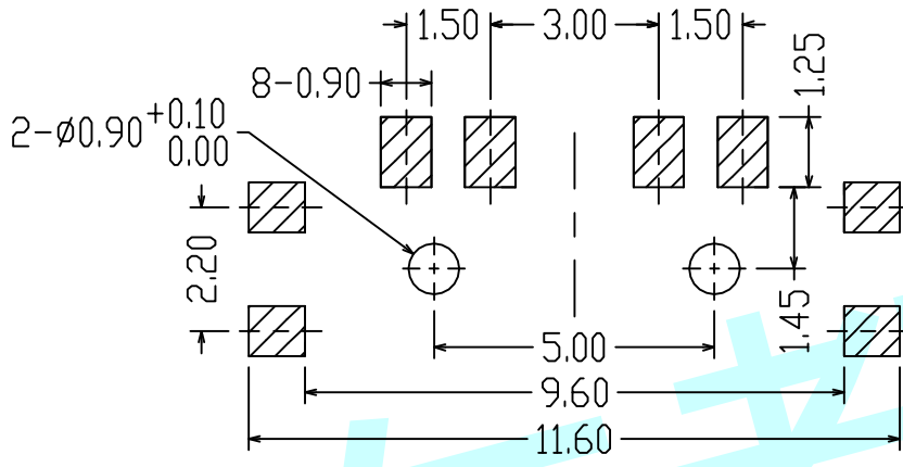
PCB Layout (Pattern Side)
