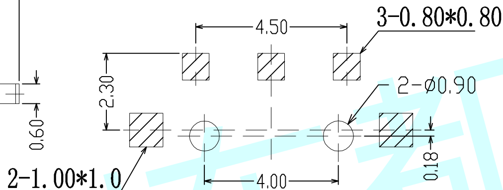
PCB LAYOUT
