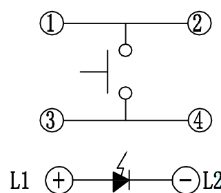
Circuit Diagram
