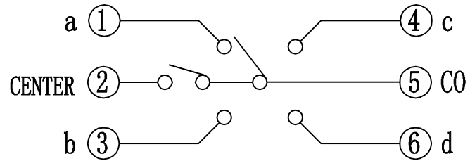
Circuit Diagram
