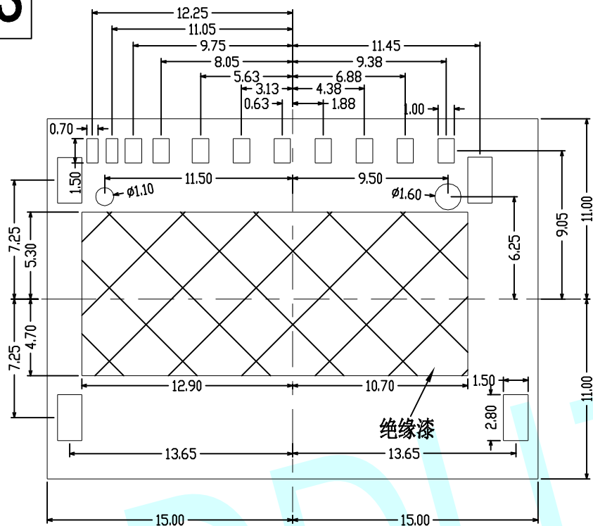
PCB LAYOUT (TOLERANCE: ±0.05)
