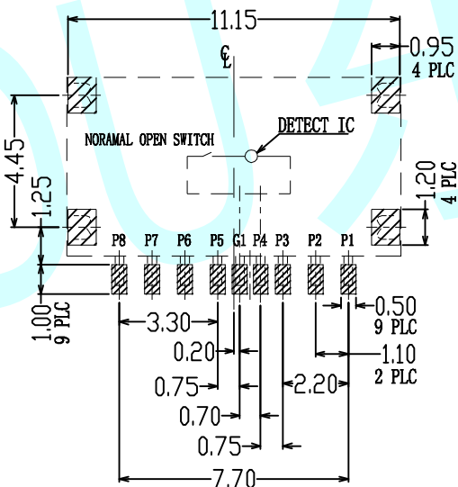
RECOMMENDED PCB LAYOUT TOL: ±0.05
